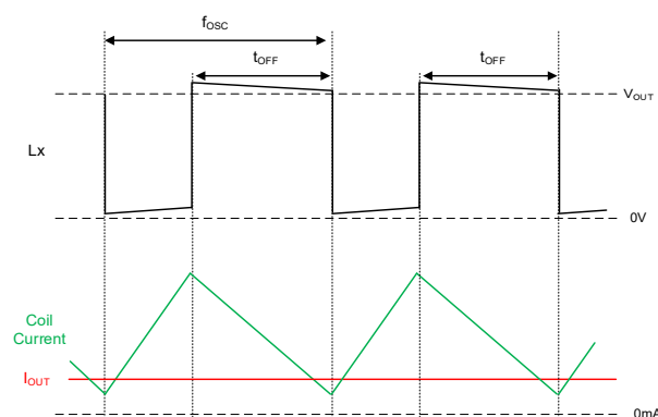
XCL104 Series : Example of heavy load operation
