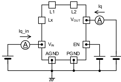
< Circuit No.5 >
