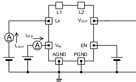
< Circuit No.8 >
