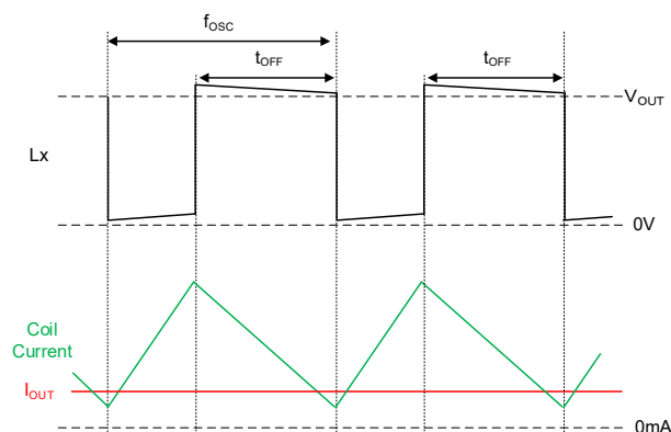
XCL105 Series: Example of heavy load operation
