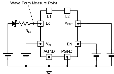
< Circuit No.8 >
