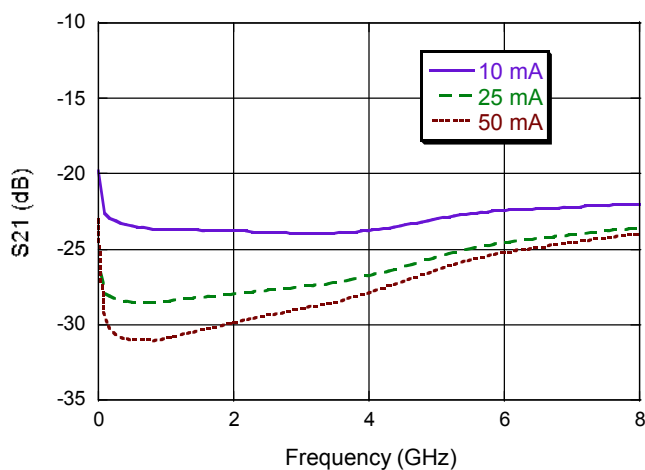
Isolation
