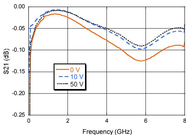
Insertion Loss
