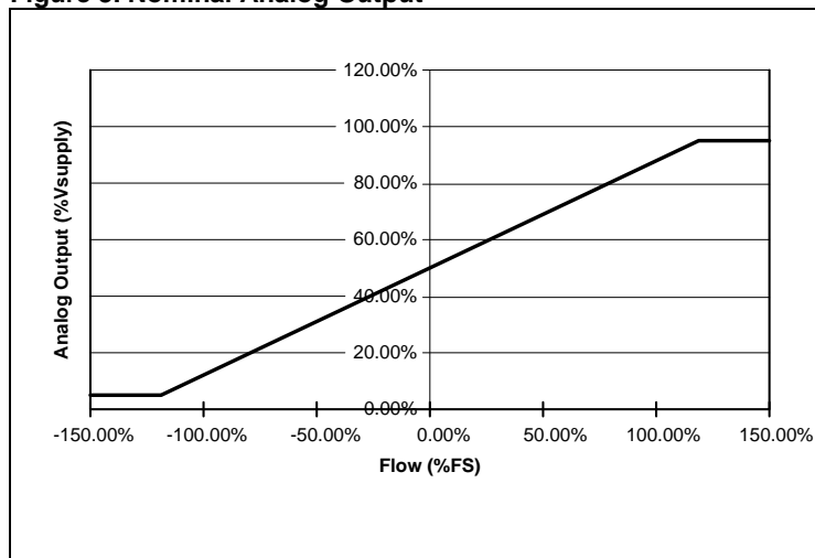
Figure 3. Nominal Analog Output
