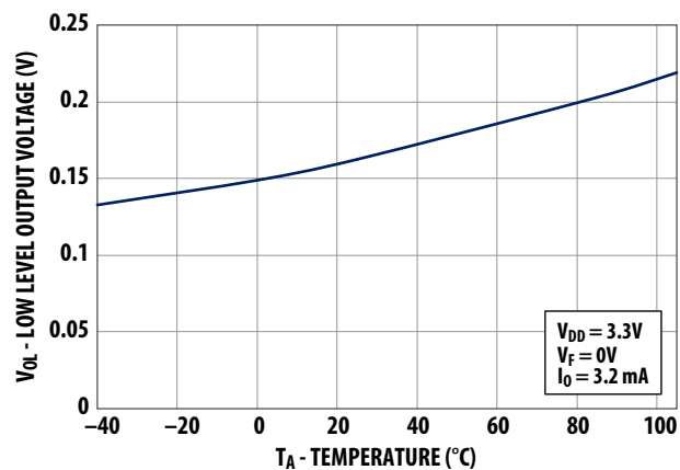
Figure 9: Logic Low Output Voltage vs. Temperature
