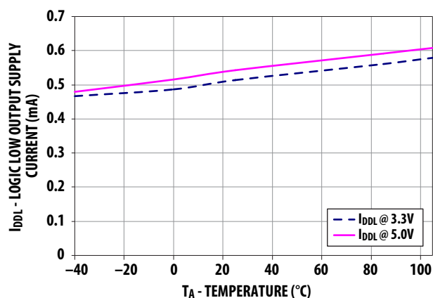
Figure 11: Logic Low Output Supply Current vs. Temperature
