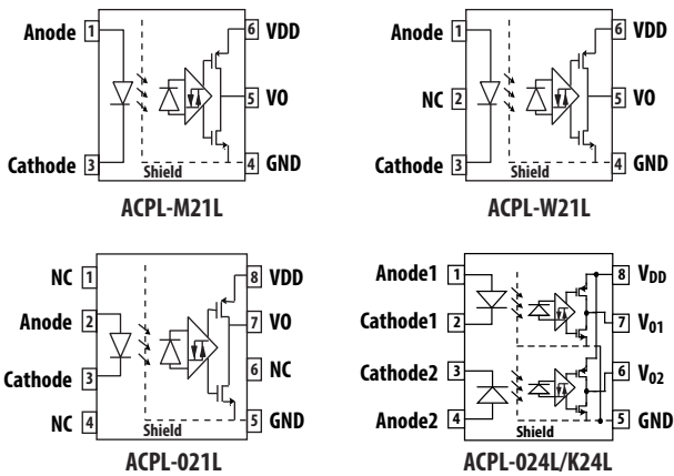
Figure 1: Functional Diagram
