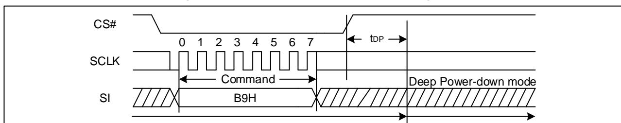
Figure 12-3. Deep Power-Down Sequence Diagram
