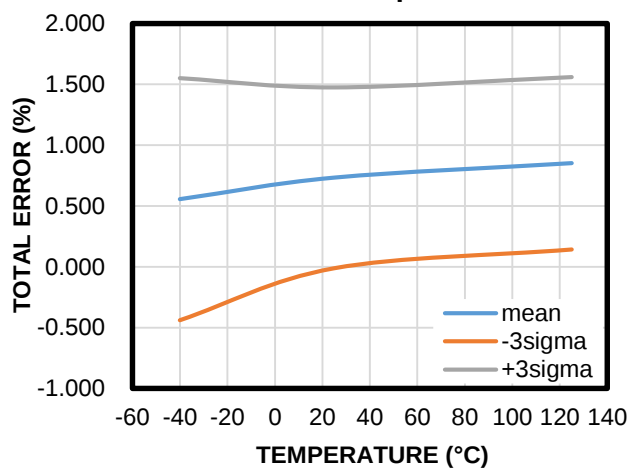
Total Error vs. Temperature
