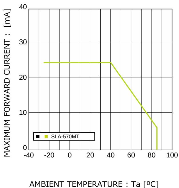
Fig.4 Derating
