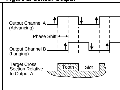
Figure 2. Sensor Output
