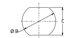
I/O Connector Recommended Cutout
