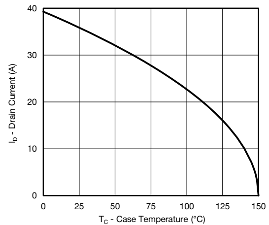
Current Derating
