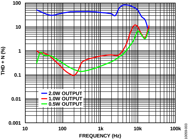
Figure 3. THD + N Performance of Circuit Using 5 V Power Supply, 4 Ω + 15 μH Load, Gain = 3 dB
