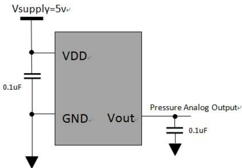
FIGURE 1: CPS175 ANALOG OUTPUT CIRCUIT
