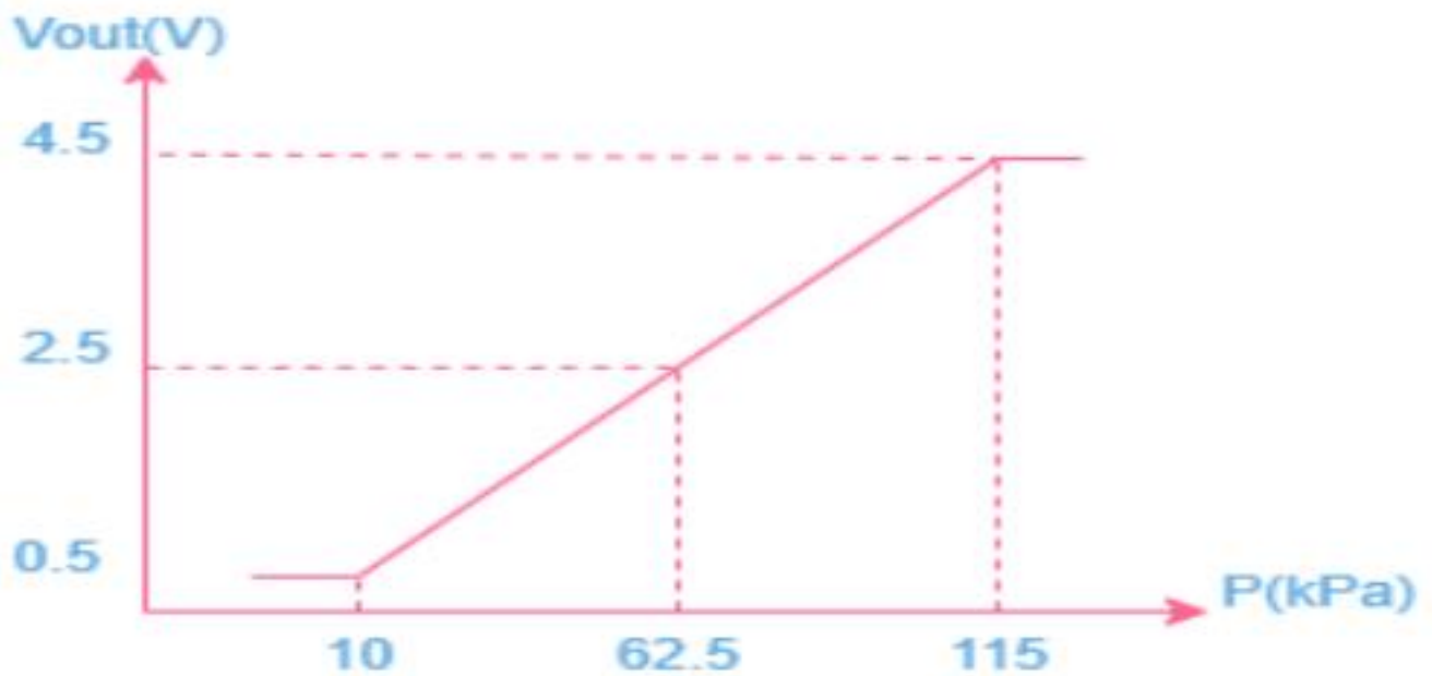
FIGURE 2: EXAMPLE OF ANALOG OUTPUT VS. PRESSURE
