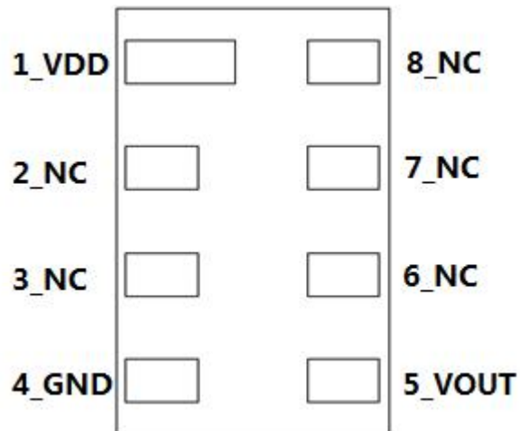
FIGURE 3: CPS175 PACKAGE PIN LAYOUT
