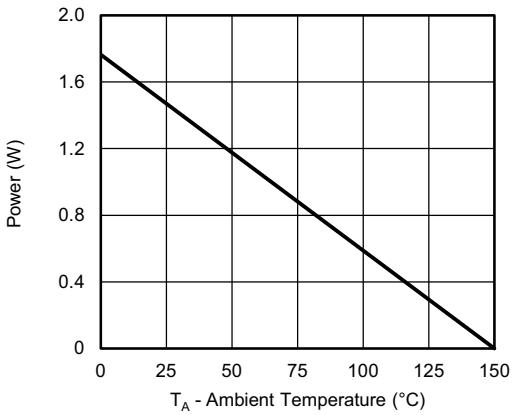
Power, Junction-to-Ambient
