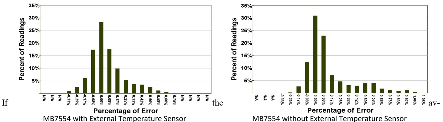
MB7554 with External Temperature Sensor and Fan
