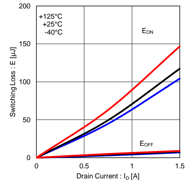
Figure 34. High Side Switching Loss (VDC=300V)
