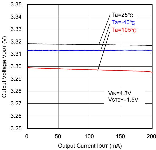
Figure 17. Load Regulation
