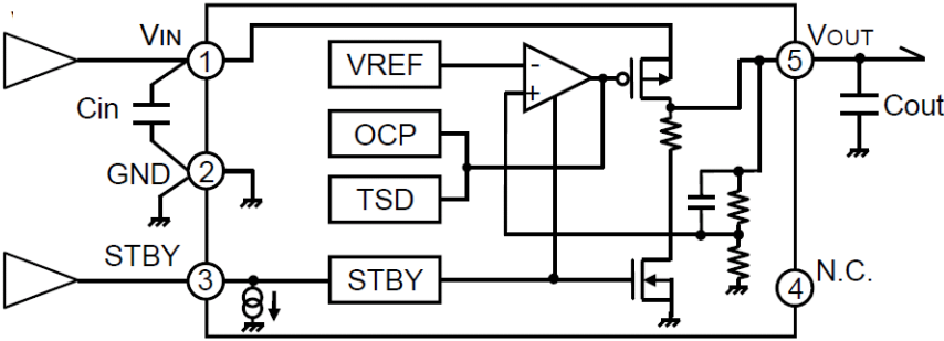
Figure 2. Block diagram
