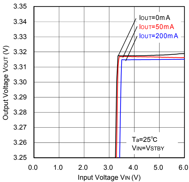
Figure 15. Line Regulation
