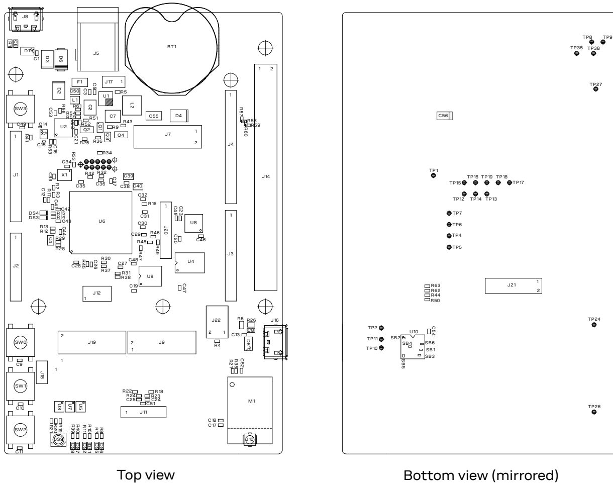
Figure 22: Component layout
