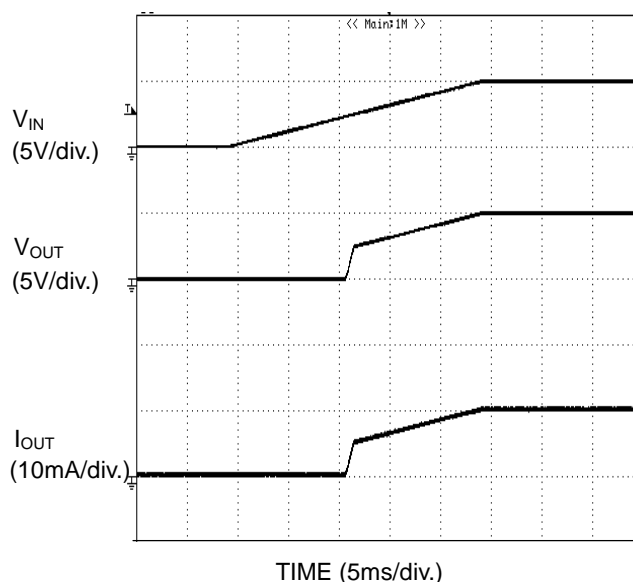
Figure 61. UVLO Response Increasing V_{IN}
