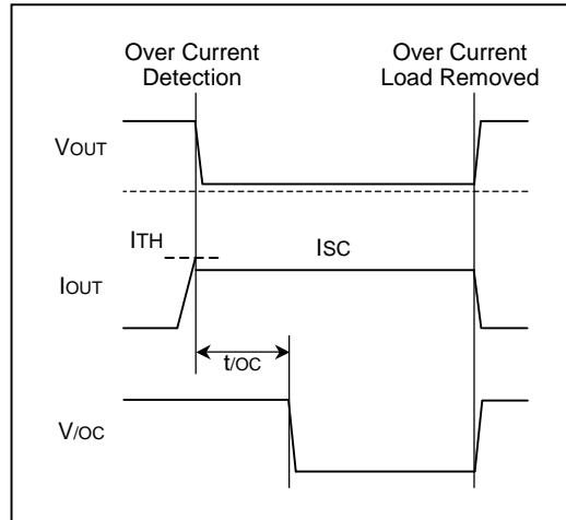
Figure 81. Over-Current Detection
