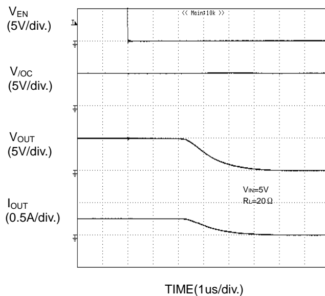
Figure 73. Output fall characteristic
