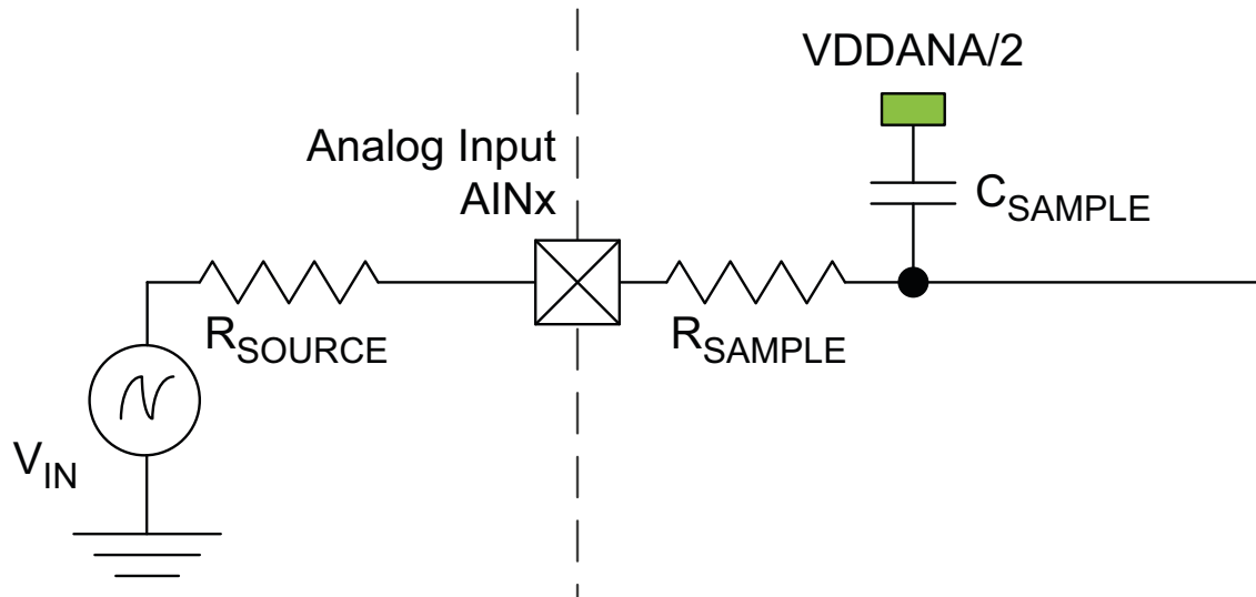
Figure 36-5. ADC Input
