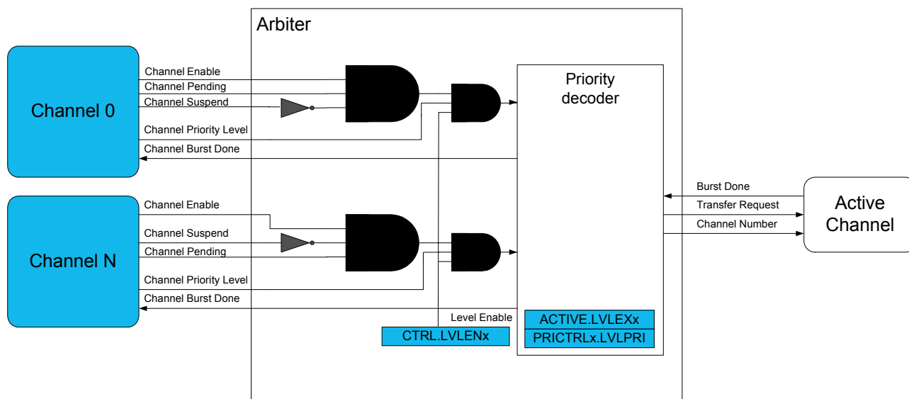
Figure 19-4. Arbiter Overview
