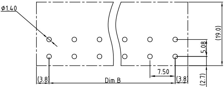
PCB LAYOUT
