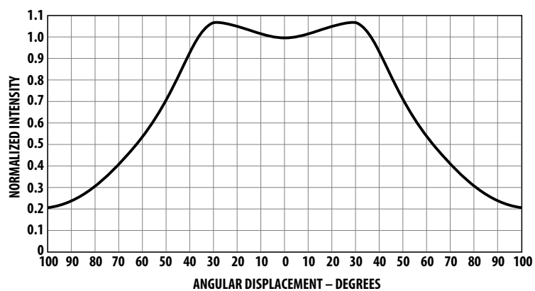
Figure 10: Relative Luminous Intensity vs. Angular Displacement for 125° Device
