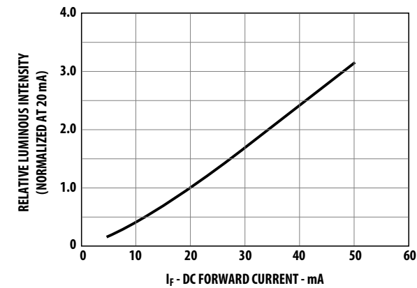
Figure 5: Relative Luminous Intensity vs. DC Forward Current, HLMT-xxxx
