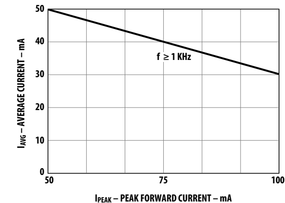
Figure 7: Maximum Average Current vs. Peak Forward Current, HLMA-xxxx
