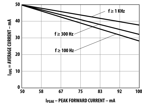
Figure 8: Maximum Average Current vs. Peak Forward Current, HLMT-xxxx
