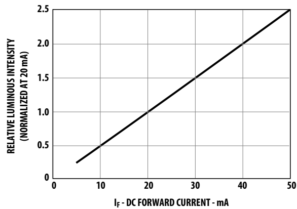
Figure 4: Relative Luminous Intensity vs. DC Forward Current, HLMA-xxxx
