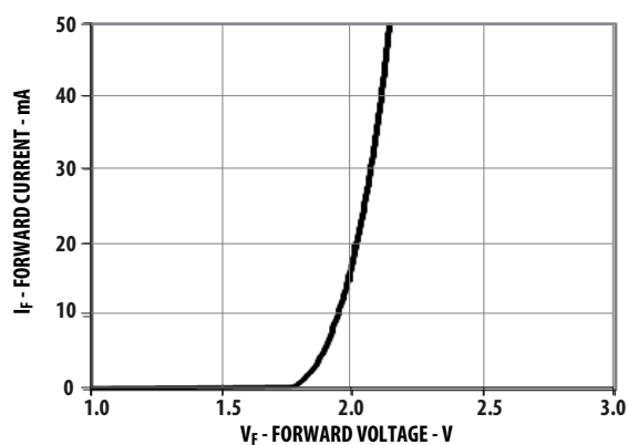
Figure 3: Forward Current vs. Forward Voltage, HLMT-xxxx
