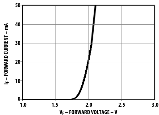
Figure 2: Forward Current vs. Forward Voltage, HLMA-xxxx
