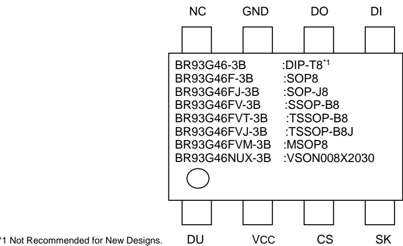
Figure 3. Pin Configuration
