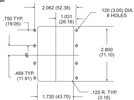
- 33 FRONT MOUNT
