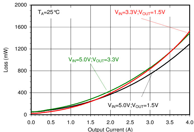
Total Loss (Forced PWM)
