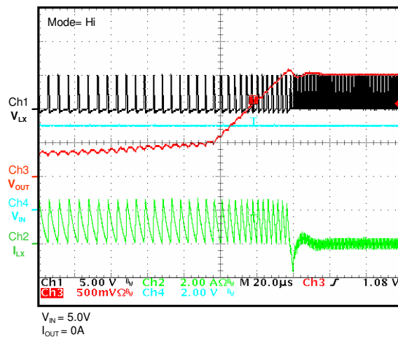
Recovery from OCP ( V_{OUT}=1.5\text{V} )
