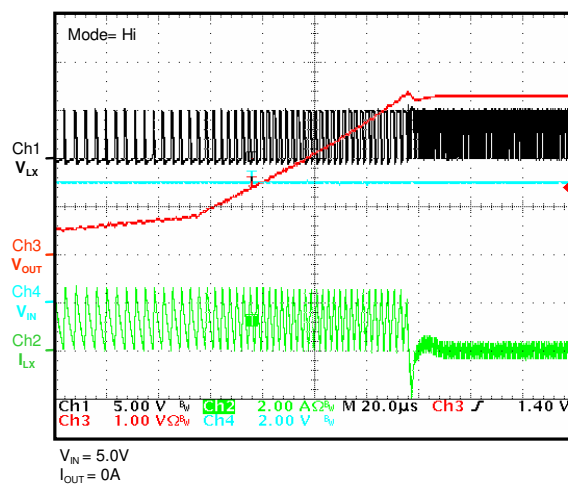
Recovery from OCP ( V_{OUT}=3.3\text{V} )
