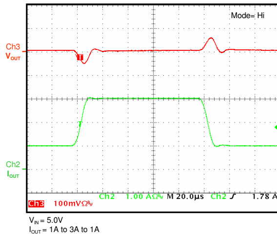
Transient Response ( V_{OUT}=3.3\text{V} , I_{STEP}=2\text{A} )
