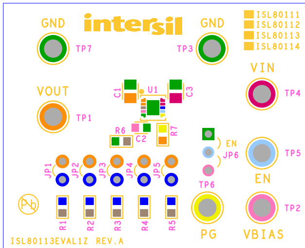
FIGURE 4. SILKSCREEN TOP
