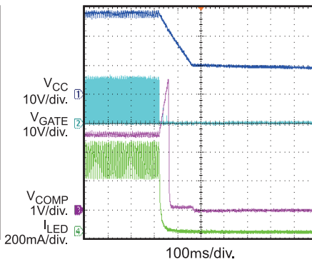
V_{IN} Shut-Down
