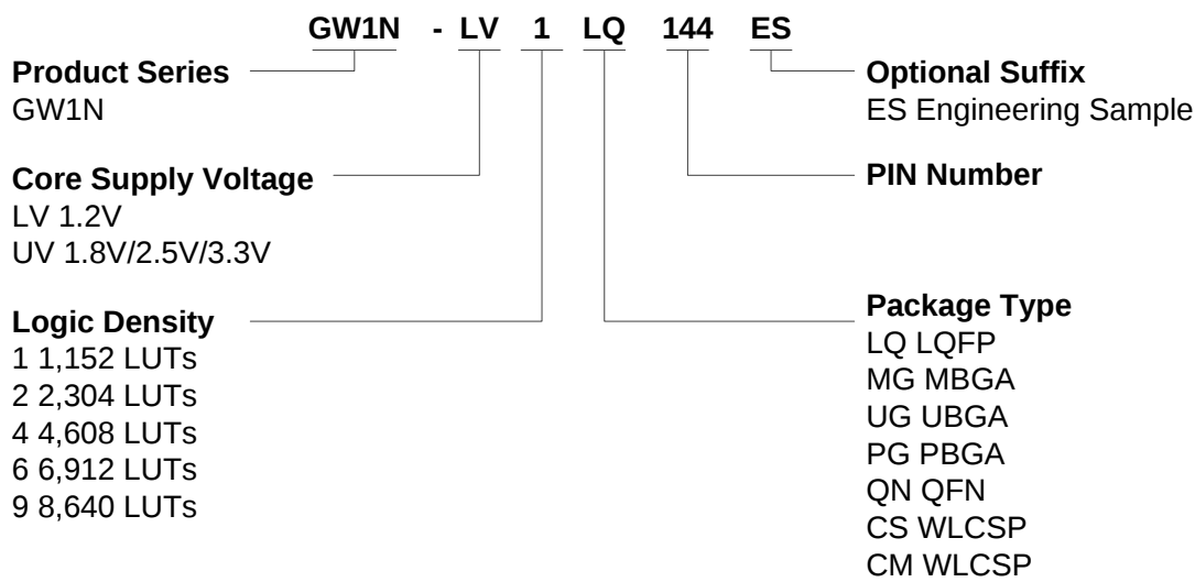
Figure 5-1 Part Naming-ES
