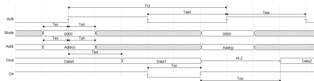
Figure 4-1 Read Mode
