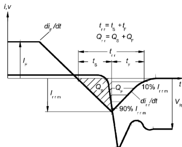
Figure 4. Definition of diode switching characteristics
