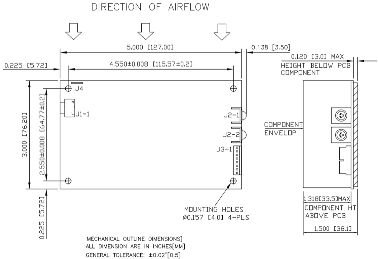
Figure 2. Mechanical Drawing
