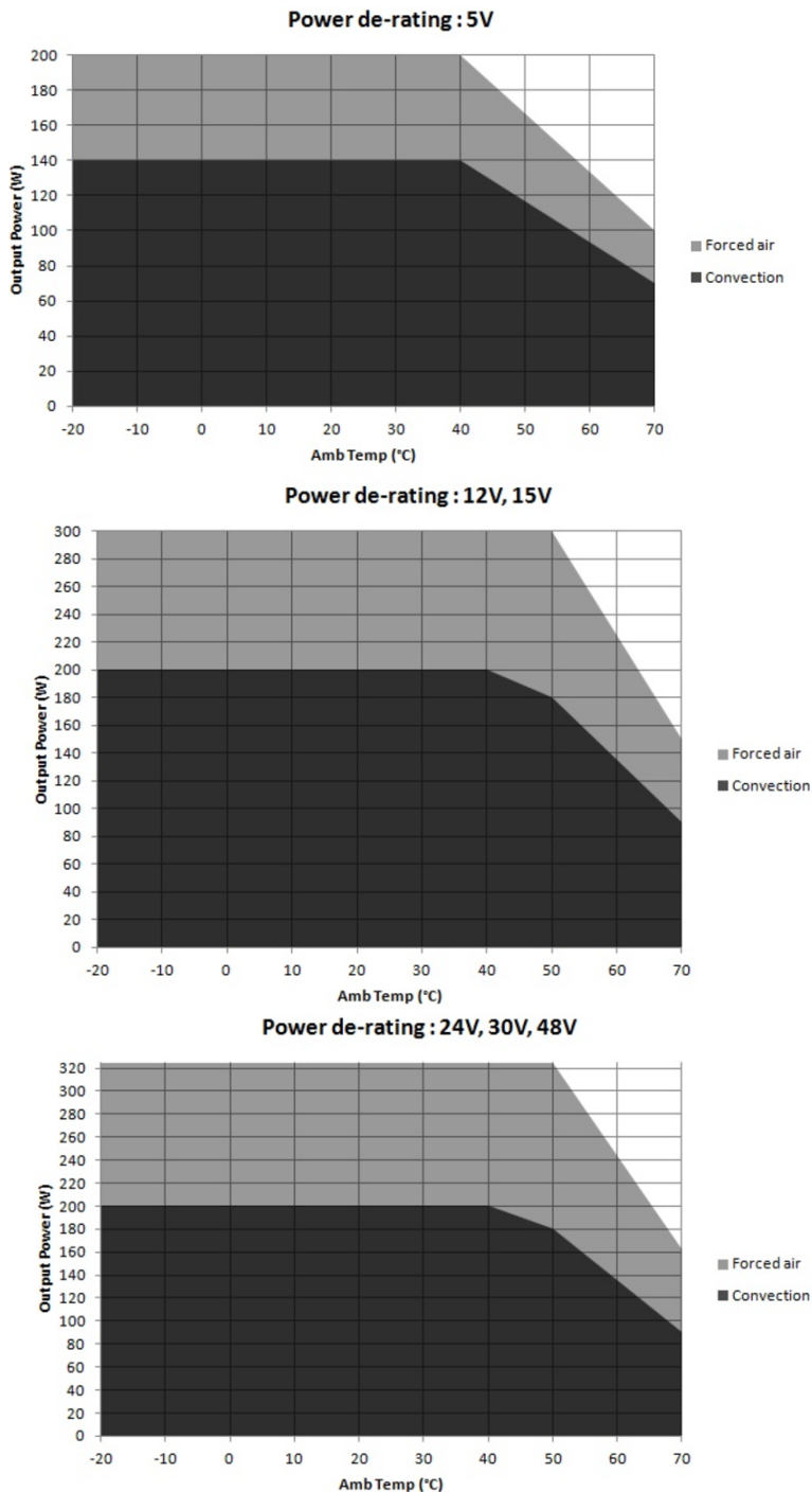
Figure 1. Derating Curves
