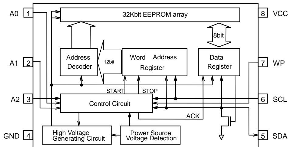
Block Diagram
