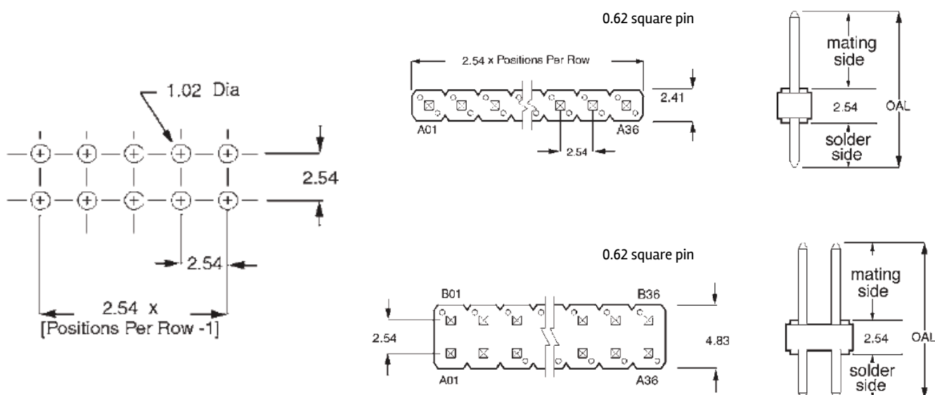
Recommended PCB Layouts Dimensions in mm
