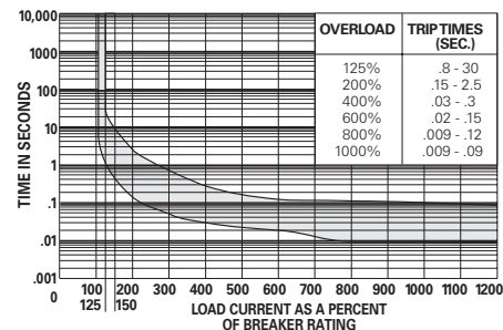
CURVE 13 HIGH INRUSH 50/60 Hz.
