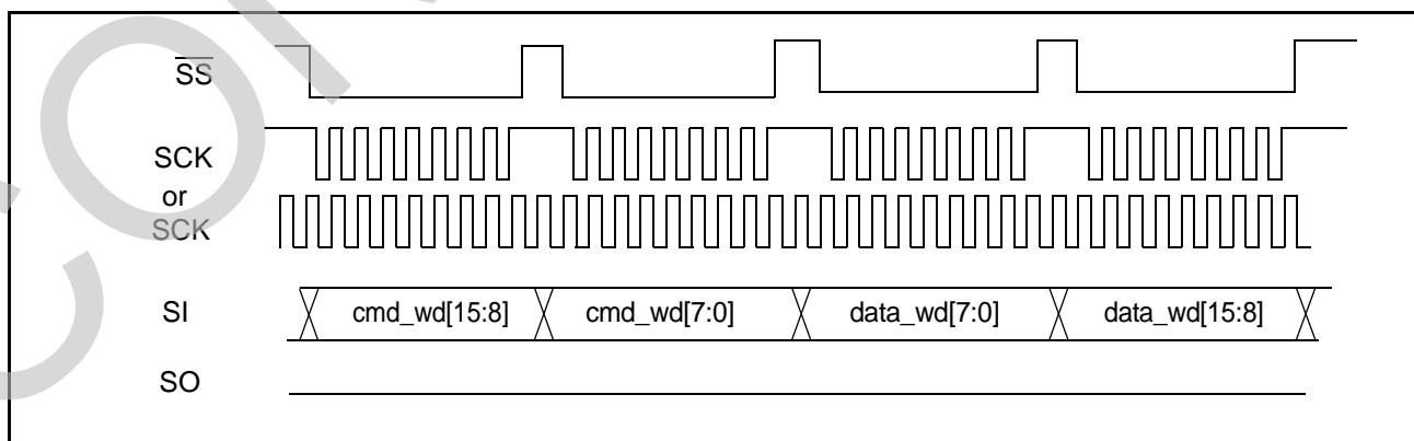
Figure 21 - One Data Word Write in Byte Framing Mode with Byte Swap
