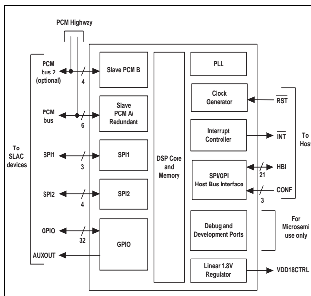
Figure 1 - Block Diagram
