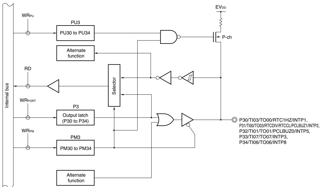
Figure 4-10. Block Diagram of P30 to P34
