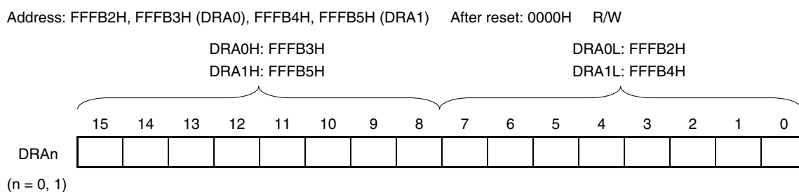
Figure 18-2. Format of DMA RAM Address Register n (DRAn)
