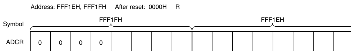
Figure 10-10. Format of 10-bit A/D Conversion Result Register (ADCR)
