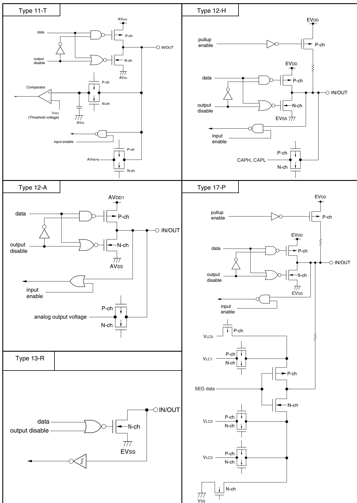
Figure 2-1. Pin I/O Circuit List (3/5)
