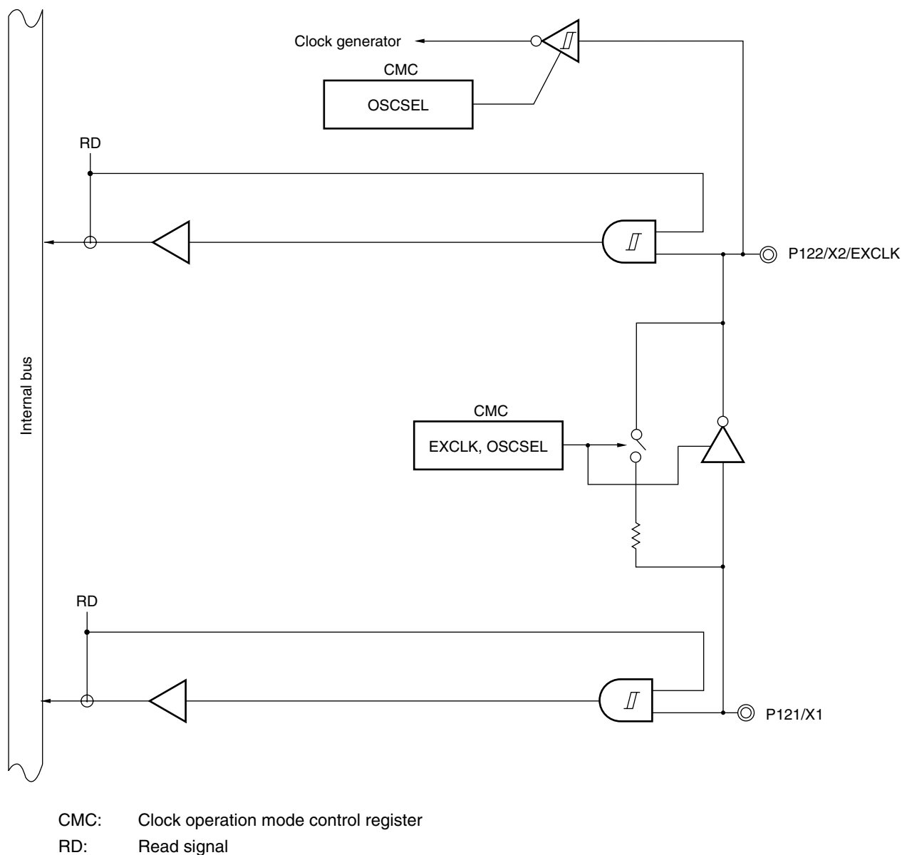
Figure 4-30. Block Diagram of P121 and P122
