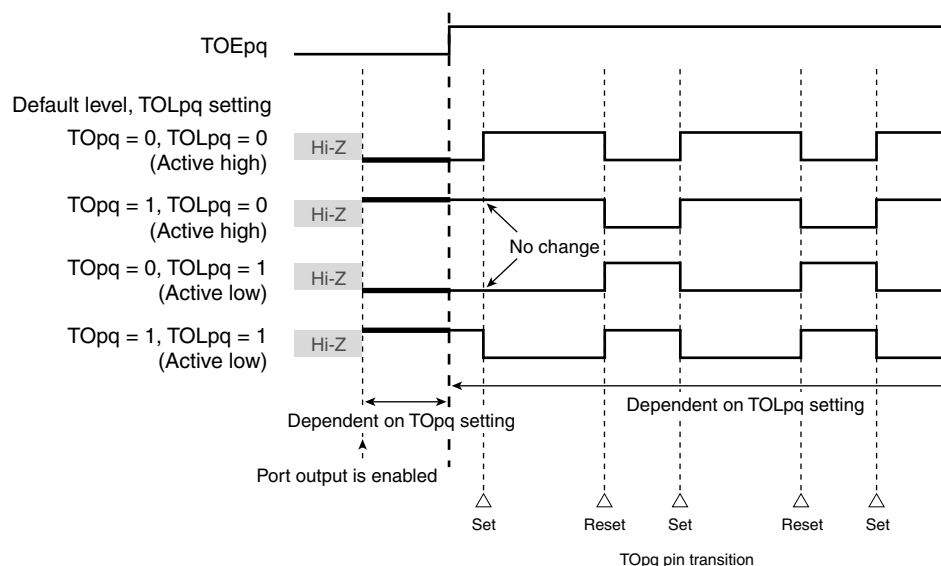
Figure 6-29. TOPg Pin Output Status at PWM Output (TOMpg = 1)
