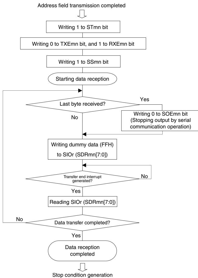
Figure 14-97. Flowchart of Data Reception
