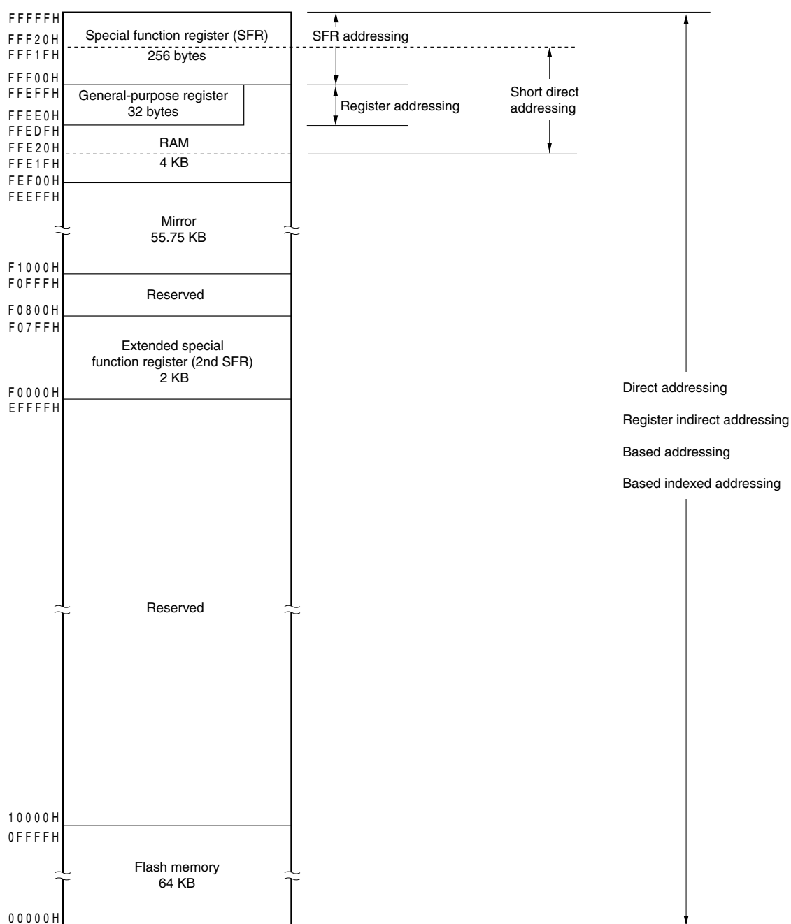
Figure 3-5. Correspondence Between Data Memory and Addressing ( \mu PD78F1500A, 78F1503A, 78F1506A, 78F1510A, 78F1513A, 78F1516A)
