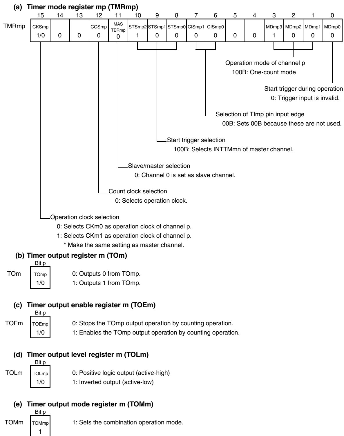
Figure 6-65. Example of Set Contents of Registers When One-Shot Pulse Output Function Is Used (Slave Channel)
