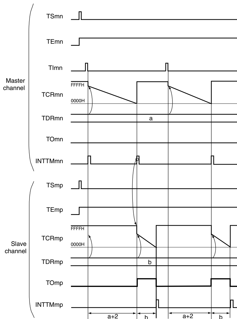
Figure 6-63. Example of Basic Timing of Operation as One-Shot Pulse Output Function (Start Trigger Tlmn Input Valid Edge)
