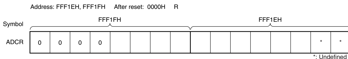
Figure 10-11. Format of 12-bit A/D Conversion Result Register (ADCR)
