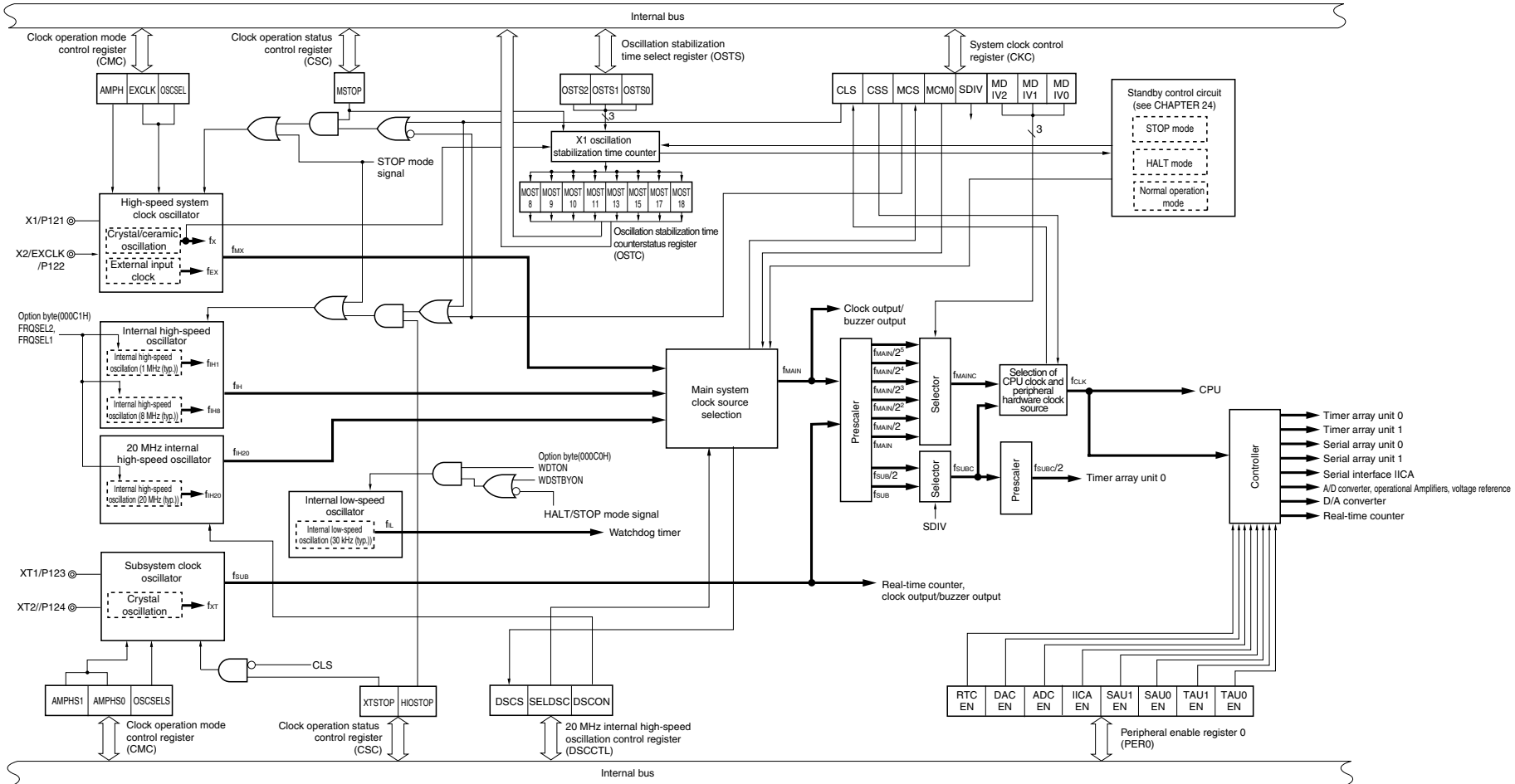
Figure 5-1. Block Diagram of Clock Generator
