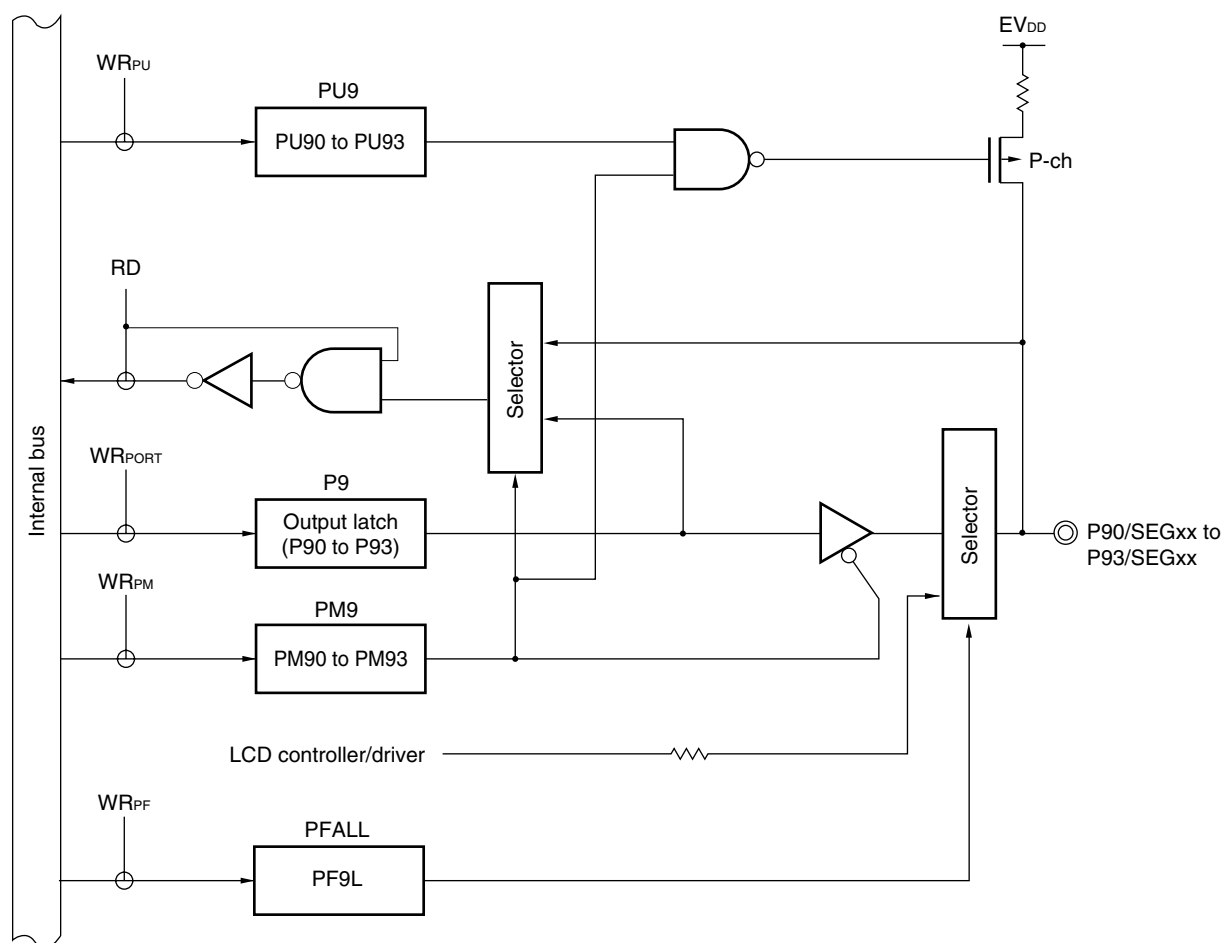
Figure 4-25. Block Diagram of P90 to P93
