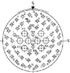
Contact Layout
