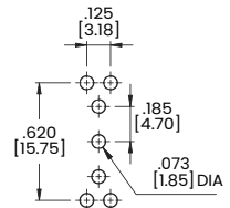
P.C.MOUNTING
