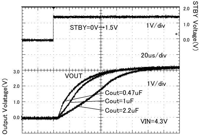
Figure 91. Startup time ( Rout = 16.5 ohm )
