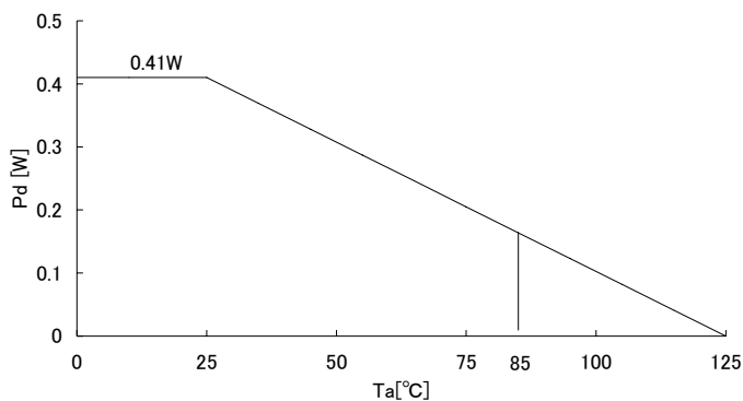
Figure 100. UCSP50L1(BUXXSA4WGWL) Power dissipation heat reduction characteristics (Reference)
