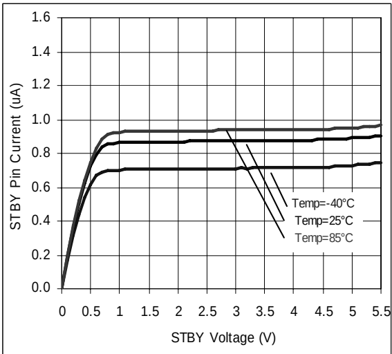
Figure 36. STBY Pin Current vs. STBY Voltage
