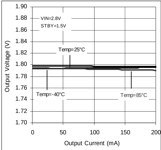
Figure 6. Load Regulation
