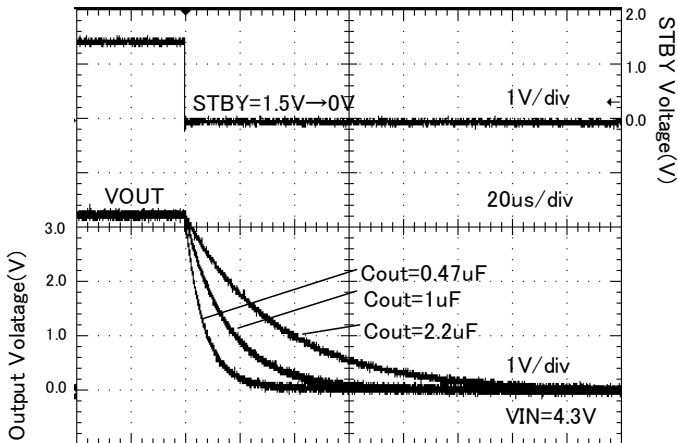
Figure 93. Discharge time ( Rout = 16.5 ohm )
