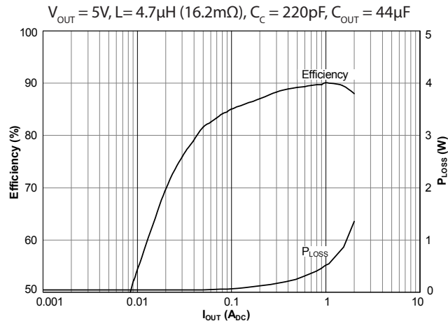
Efficiency — Power Loss (5 V_{OUT} )
