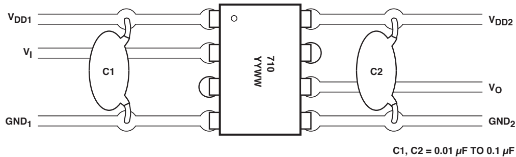
Figure 13. Recommended Printed Circuit Board layout.
