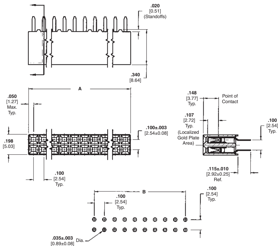
Recommended PC Board Hole Layout (for .062 [1.57] thick PC board)
