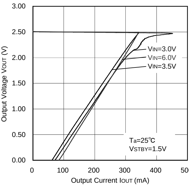
Figure 52. OCP Threshold
