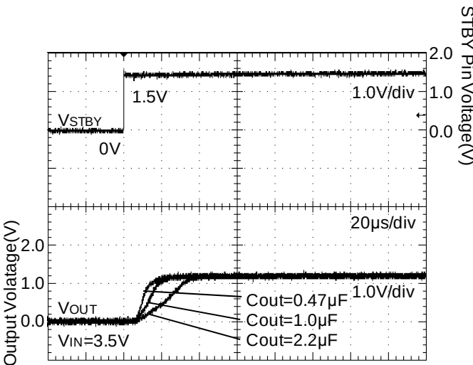
Figure 22. Startup Time (ROUT=6Ω)
