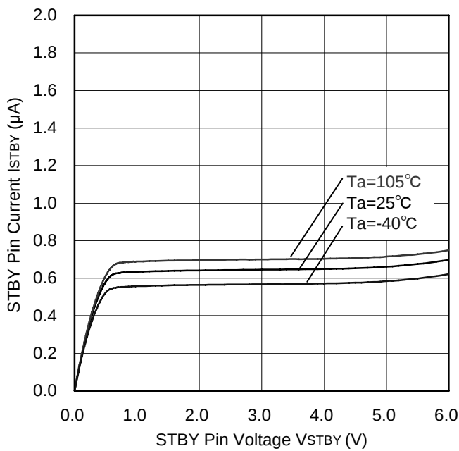
Figure 35. STBY Pin Current vs. STBY Pin Voltage
