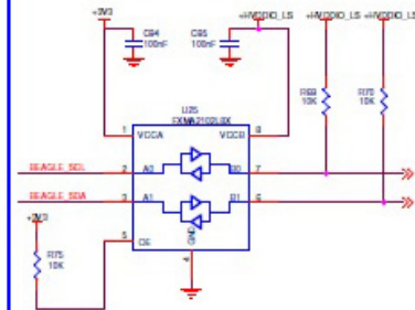
Beagle to AP0101 Adaptor board I2C level shifter
