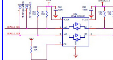
BEAGLE I2C Level shifter
