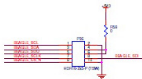
BEAGLE interface connector
