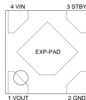
SSON004R1010 (TOP VIEW) (Note1)
