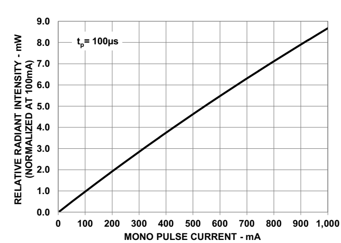
Figure 4: Relative Radiant Intensity vs. Mono Pulse Current
