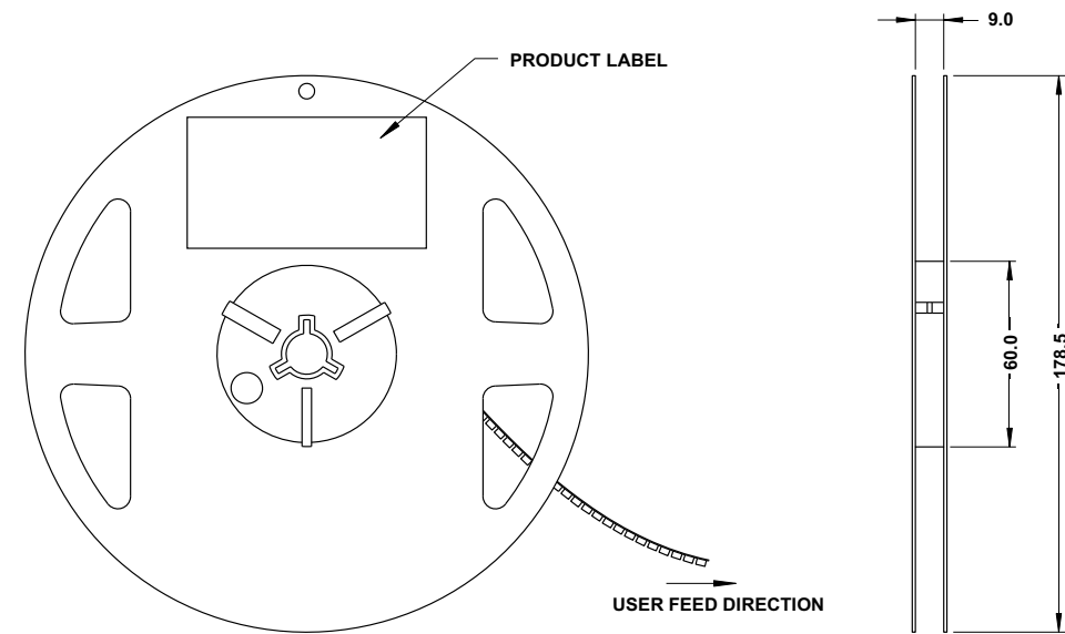
Figure 11: Reel Dimensions
