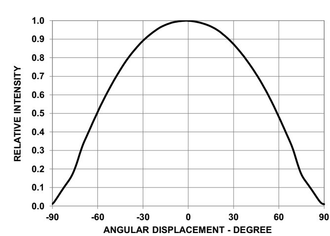
Figure 5: Radiation Pattern
