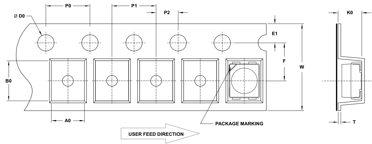
Figure 10: Carrier Tape Dimensions
