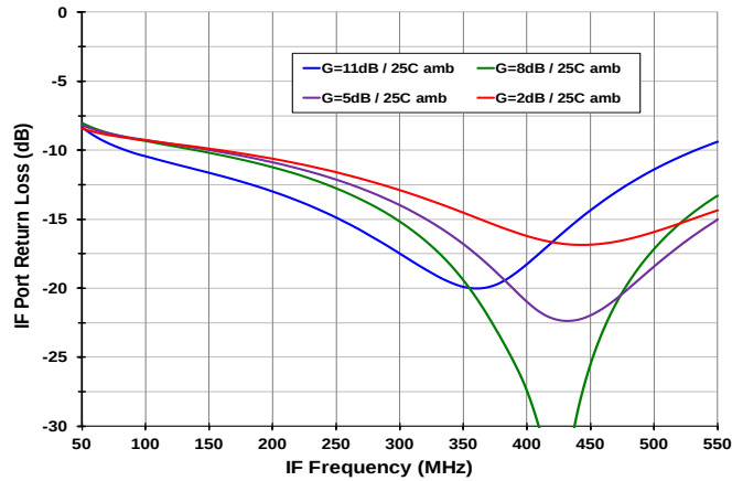
Figure 40. IF Port Return Loss vs. Gain Setting
