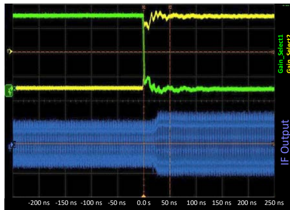
Figure 50. Gain Settling Time for 5dB to 2dB Gain Setting
