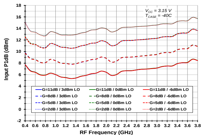
Figure 10. Input P1dB vs. LO Level and Gain Setting ( V_{CC} = 3.15 , T_{CASE} = -40^{\circ}\text{C} )
