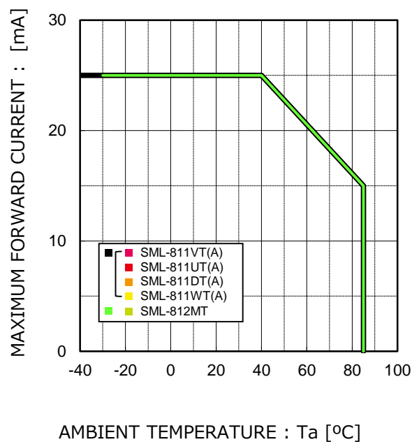
Fig.4 Derating
