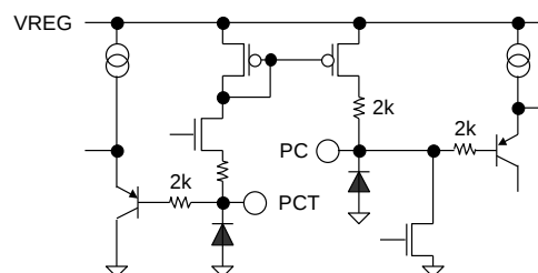
Figure 57. PC, PCT
