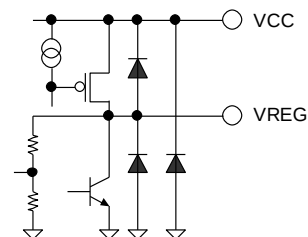
Figure 53. VREG, VCC
