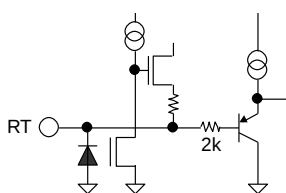
Figure 50. RT
