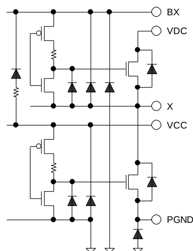
Figure 59. VCC, PGND, VDC, BX(BU/BV/BW), X(U/V/W)
