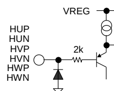
Figure 55. HXP, HXN
