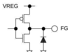
Figure 54. FG
