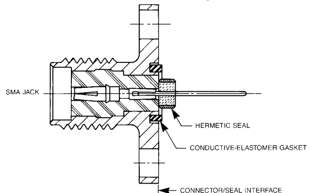
Connector / seal design—connectors for use with .012—.018" diameter pins
