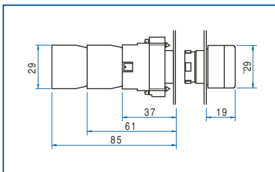
Flush Momentary
