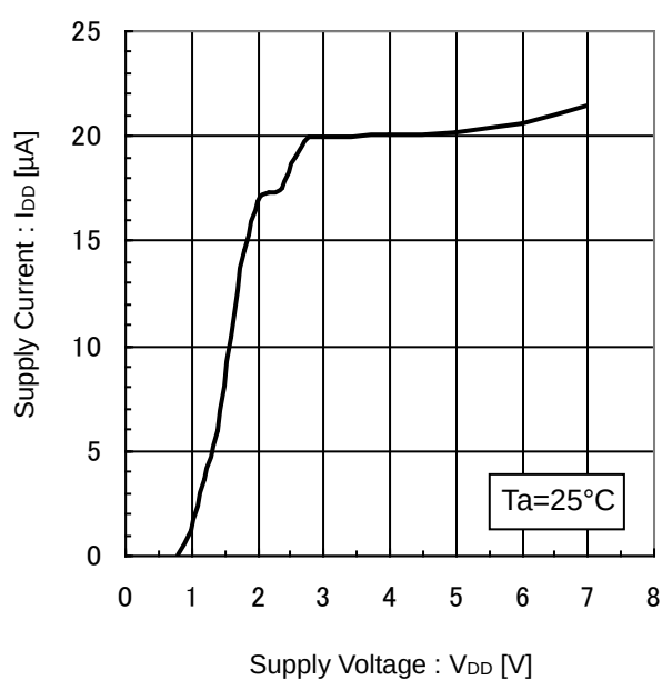
Figure 2. Supply Current vs Supply Voltage
